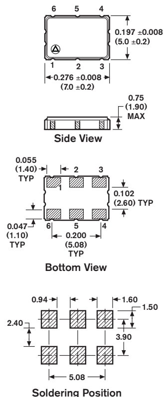
CERAMIC SMD
